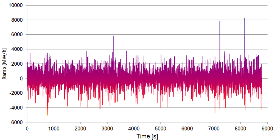
Fig. 3 Ramping needs of the net load with renewable energy.
