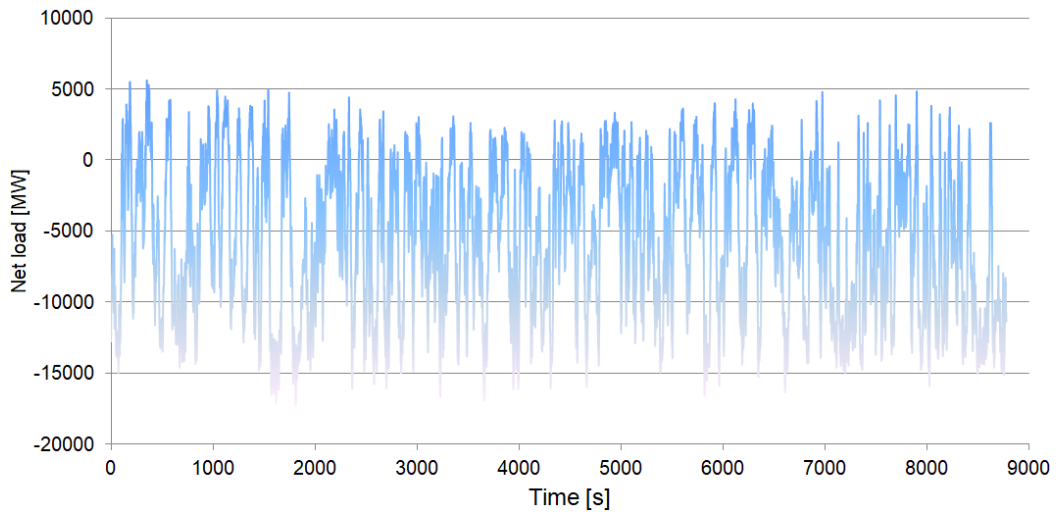
Fig. 2 Time series of net load.
