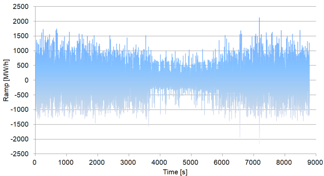
Fig. 3 Ramp needs of electricity load.
